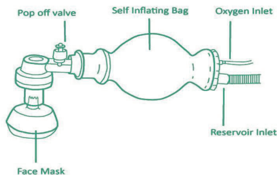
Fig. 3.1: Self inflating bag
